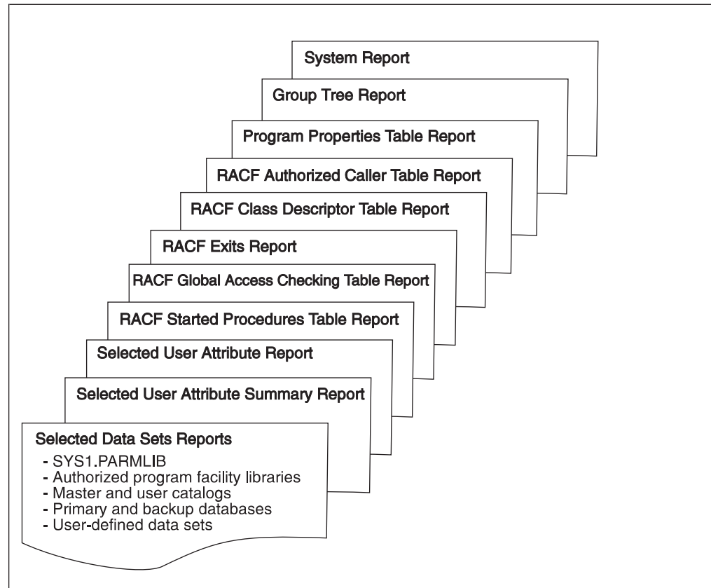
Figure 11. Reports produced by DSMON
