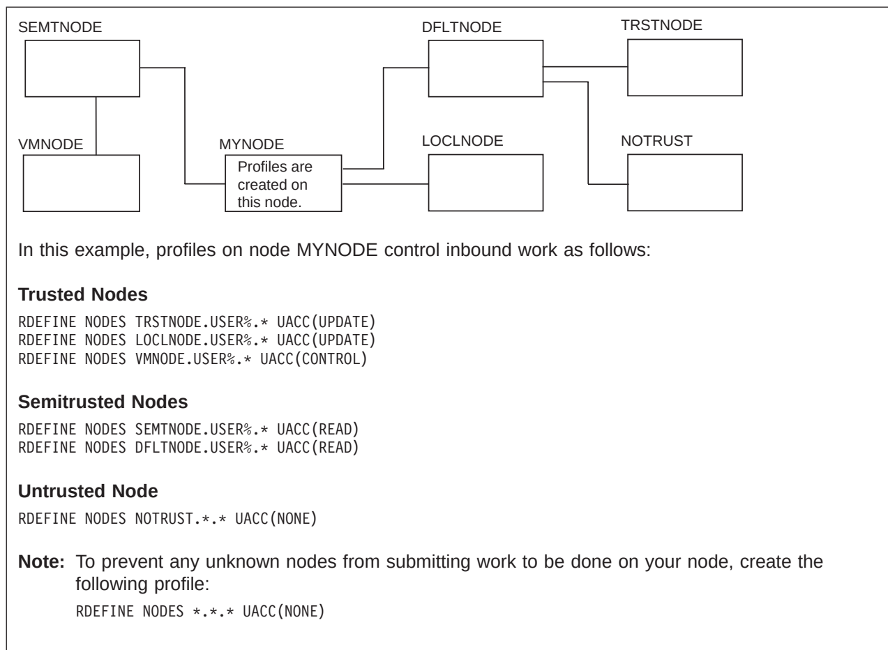
Figure 50. Example: Trusted, Semitrusted, and Untrusted Nodes
