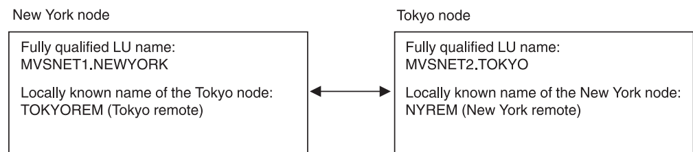
Figure 9. Example of Two Network LU Partners
