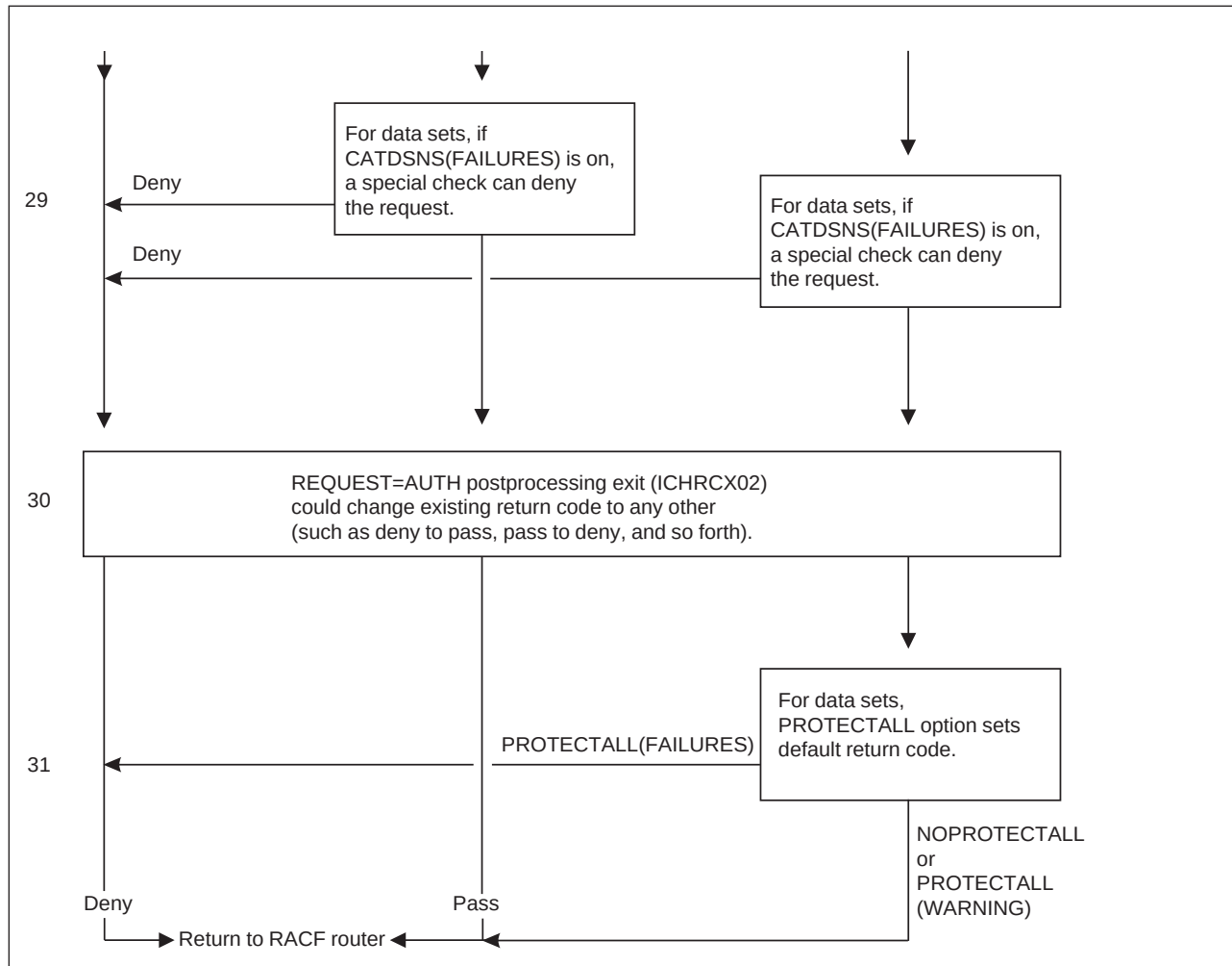
Figure 71. Process Flow of RACF Authorization Checking (Part 3 of 3)
