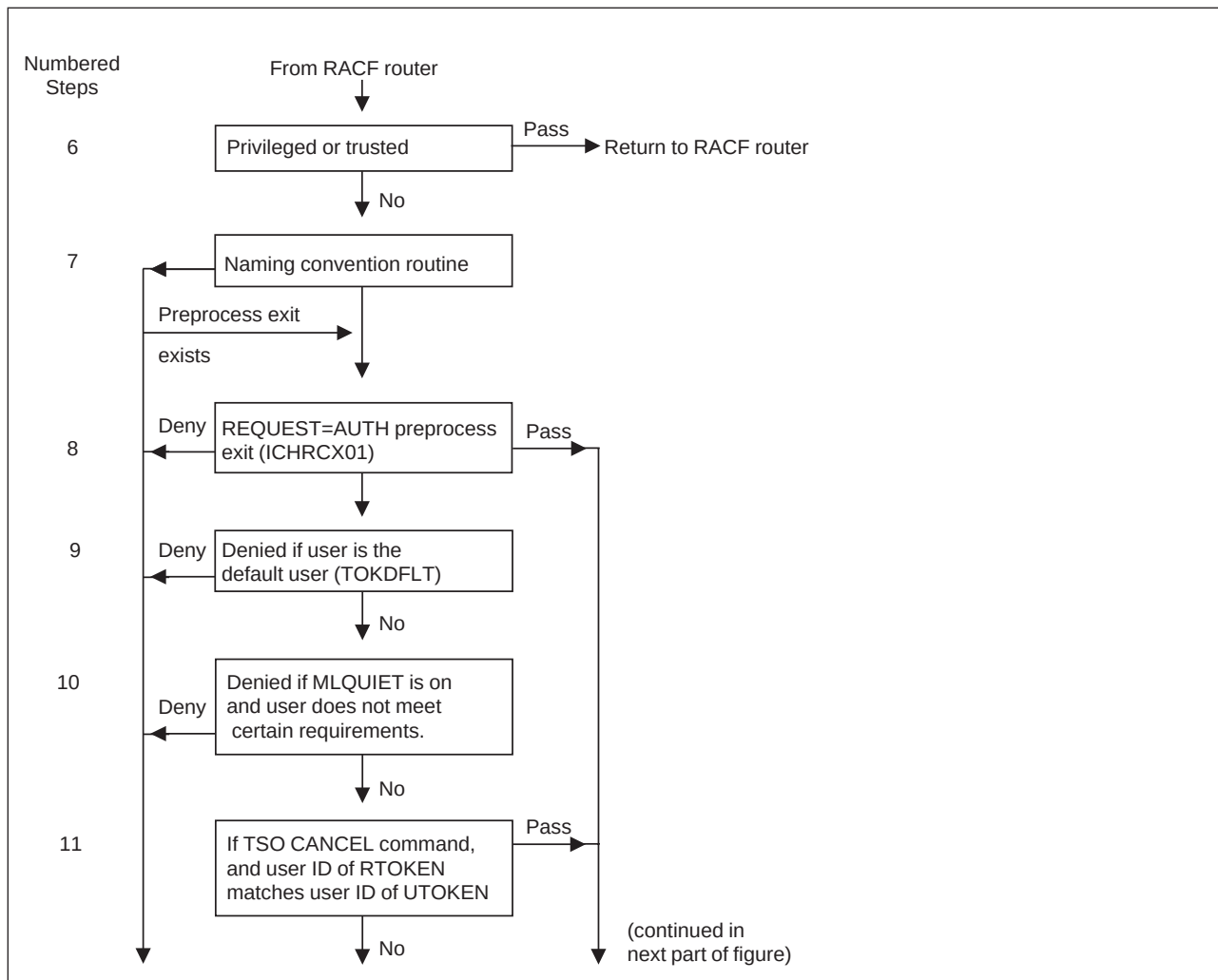
Figure 71. Process Flow of RACF Authorization Checking (Part 1 of 3)
