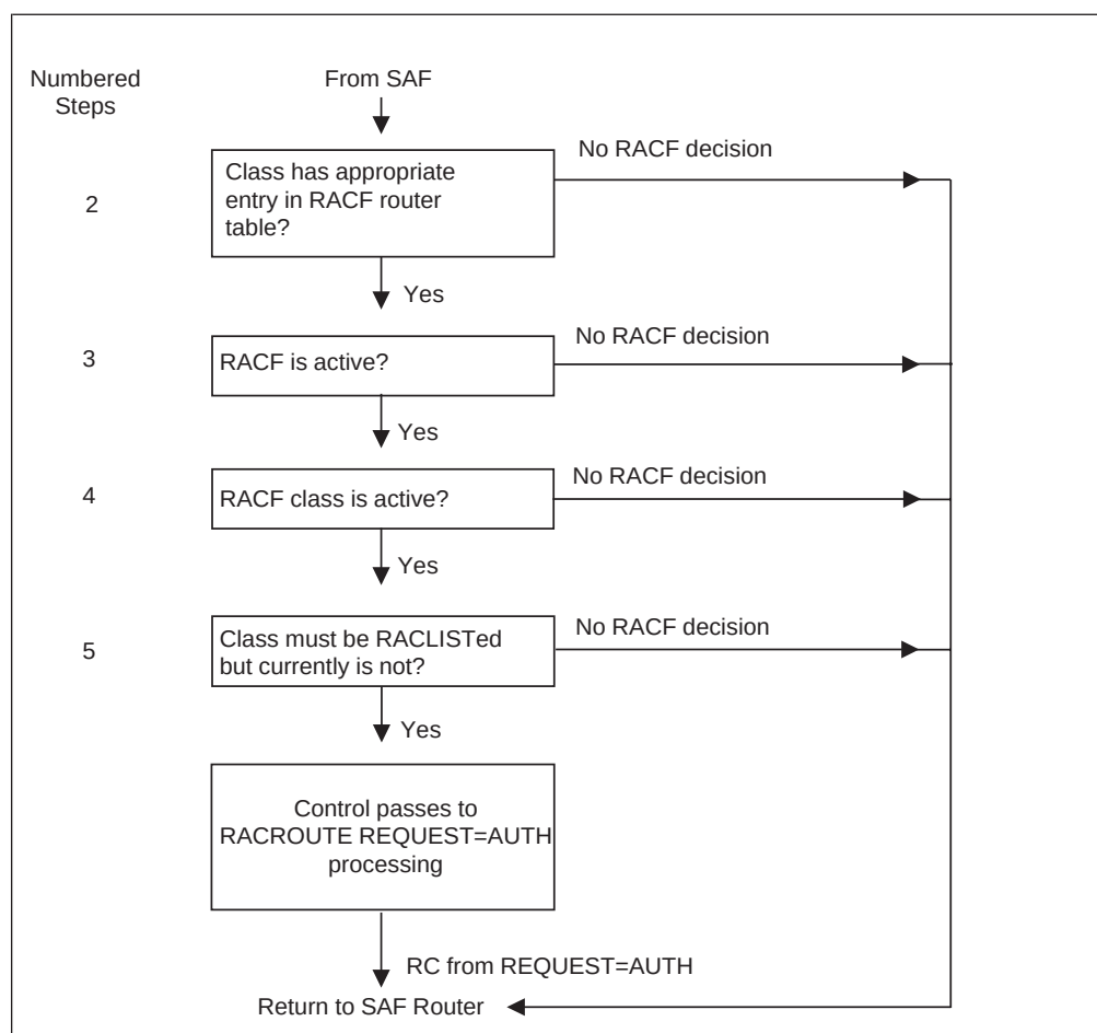
Figure 70. Process Flow of RACF Router
