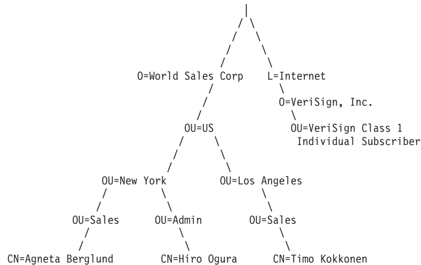
Figure 57. Example of an X.500 Directory Information Tree
