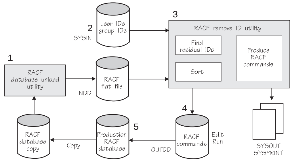
Figure 27. Using the Remove ID Utility
