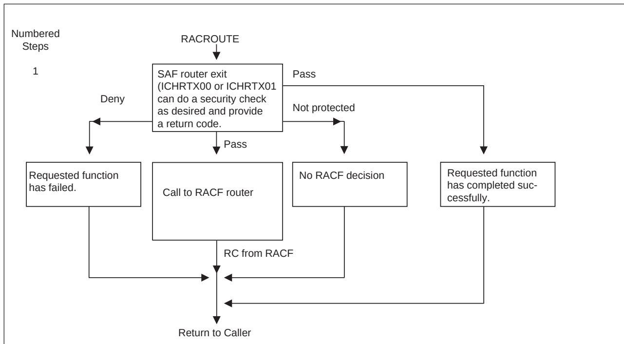
Figure 69. Process Flow of SAF Router for RACROUTE REQUEST=AUTH Requests
