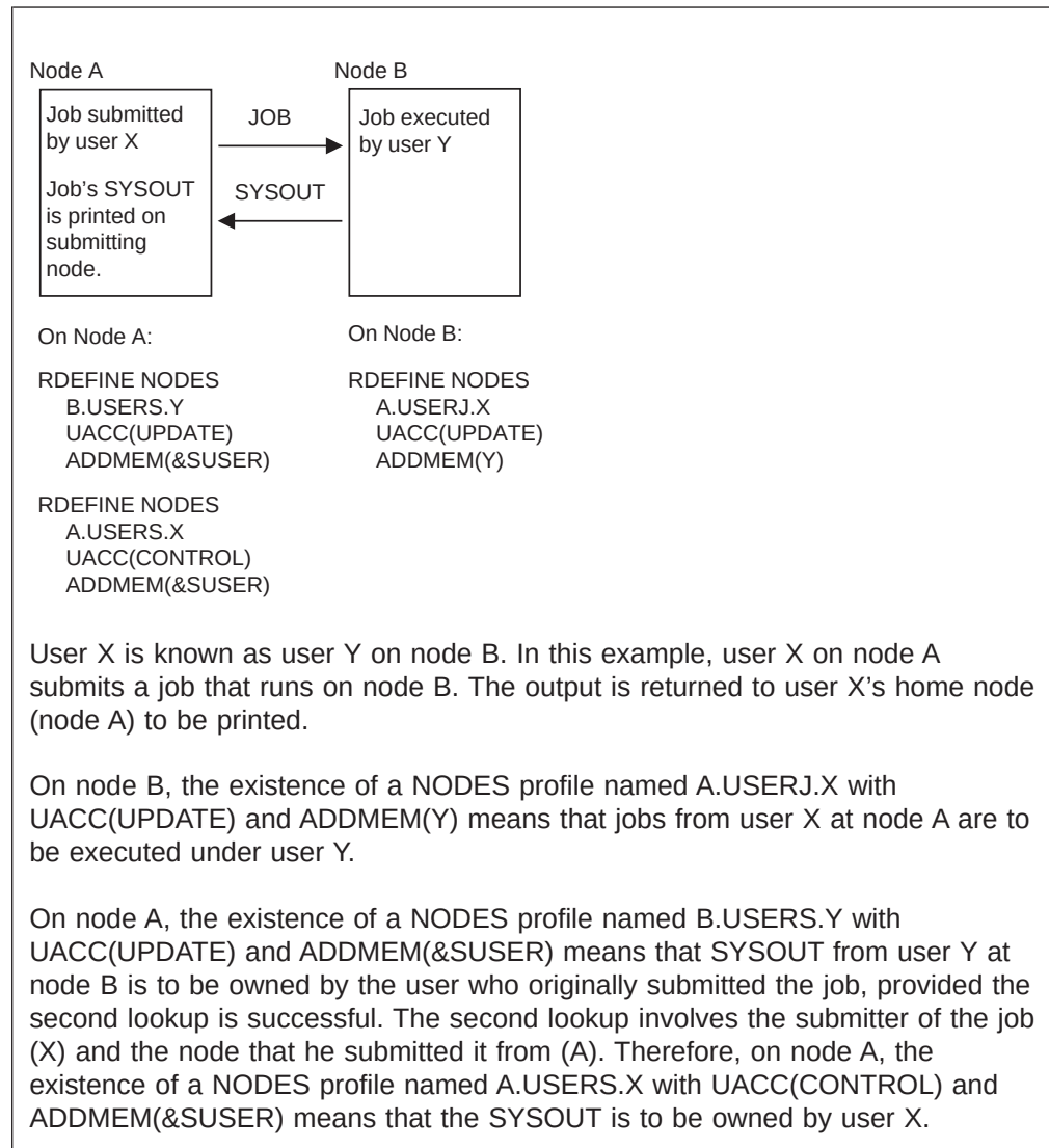
Figure 49. Example: Simple NJE User Translation Using &SUSER
