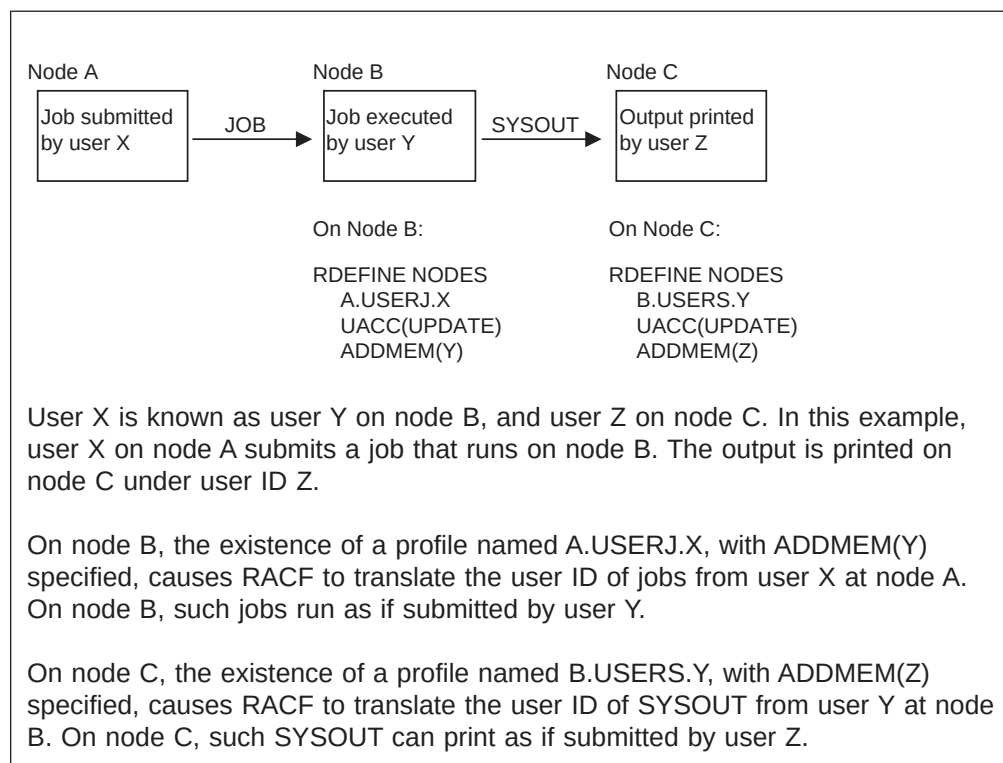
Figure 48. Example: Simple NJE User Translation
