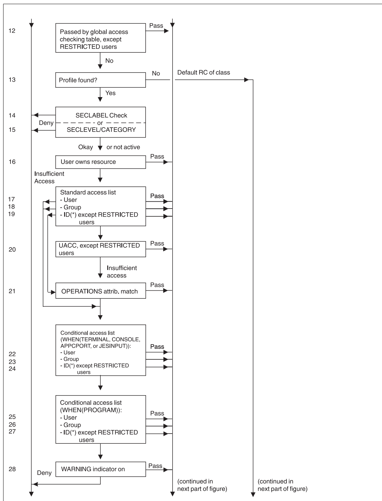
Figure 71. Process Flow of RACF Authorization Checking (Part 2 of 3)
