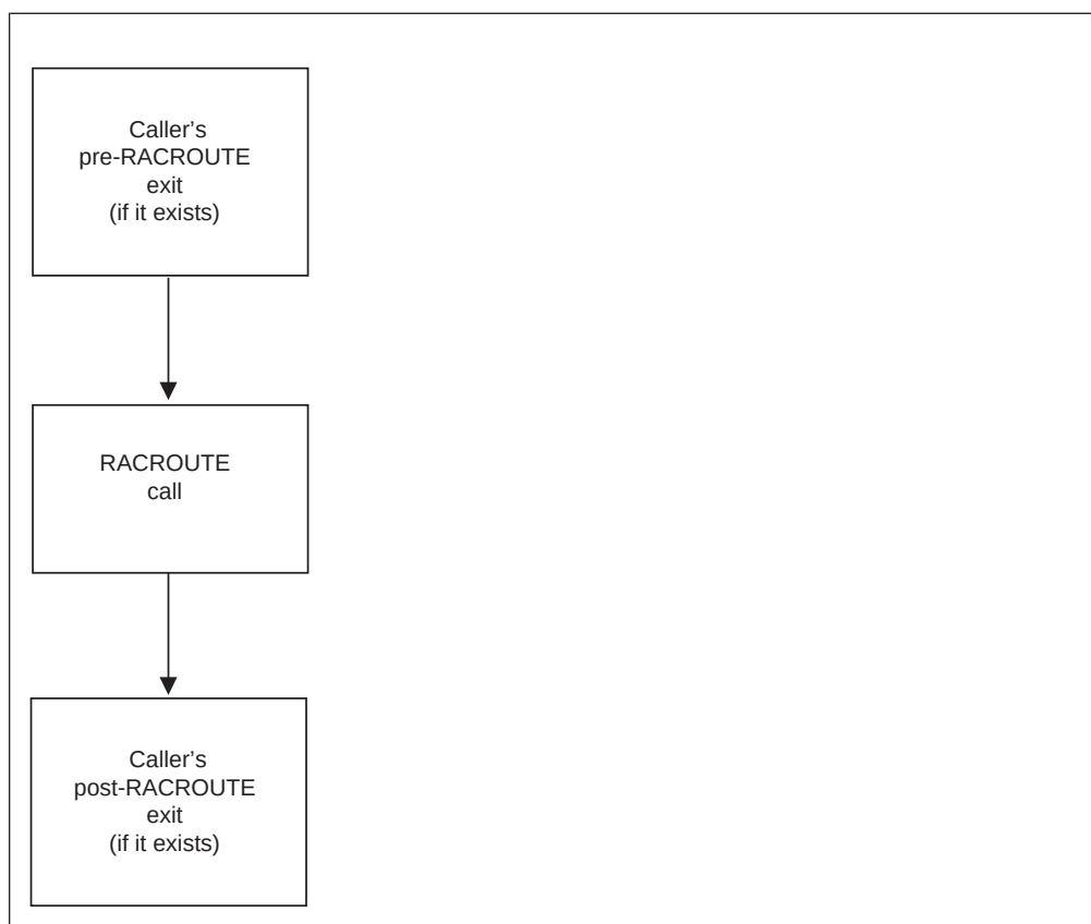
Figure 68. Process Flow of Callers of RACF for RACROUTE REQUEST=AUTH Requests
