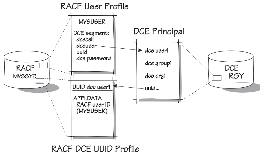
Figure 41. DCE/RACF User ID Cross Linking Example
